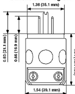
Dimensional Diagram
