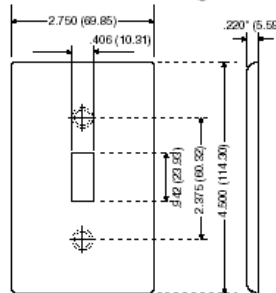
Dimensional Diagram
