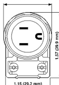
Dimensional Diagram
