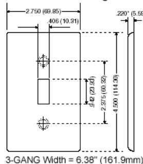
Dimensional Diagram
