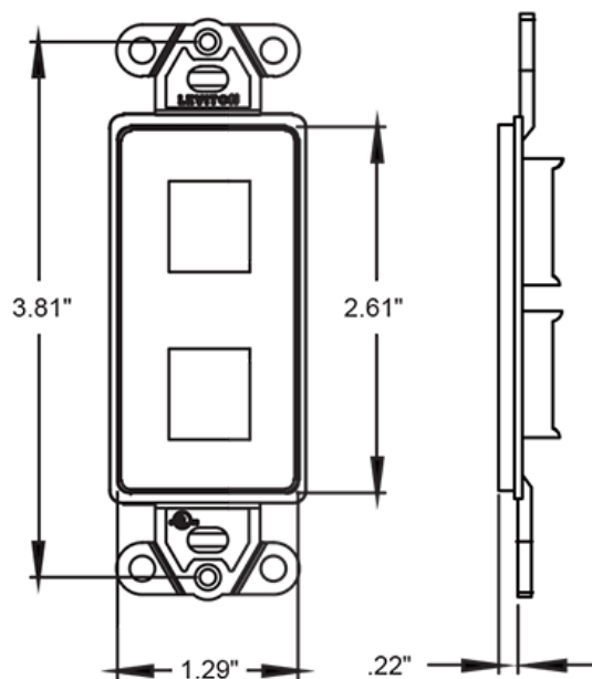
2-Port Insert
