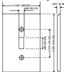
Dimensional Diagram
