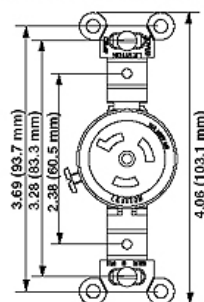
Dimensional Diagram
