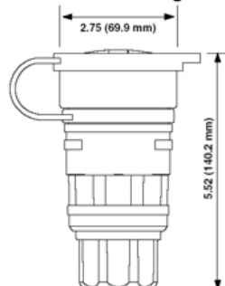
Dimensional Diagram
