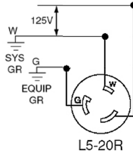
Wiring Diagram
