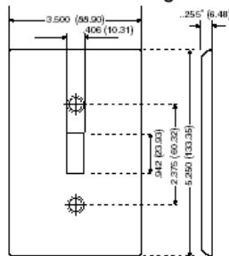
Dimensional Diagram
