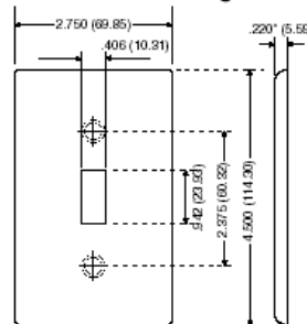
Dimensional Diagram
